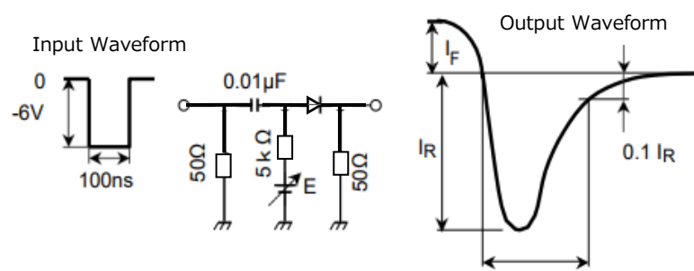
Forward and reverse voltage operation
