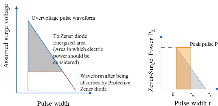
Figure. 3.3 Example of derivation of pulse width by approximating square wave from surge waveform
