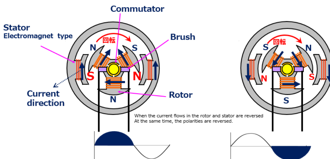
Figure 1.2 Universal motor
