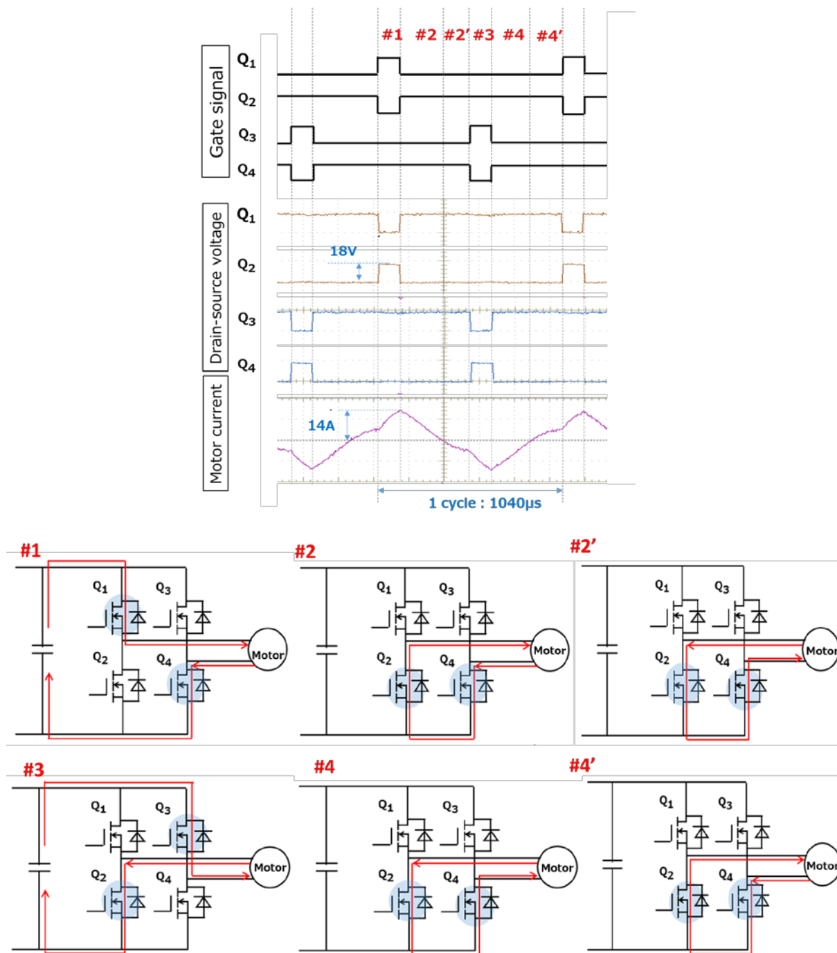
(a) Basic circuit operations and waveforms at a low suction level
