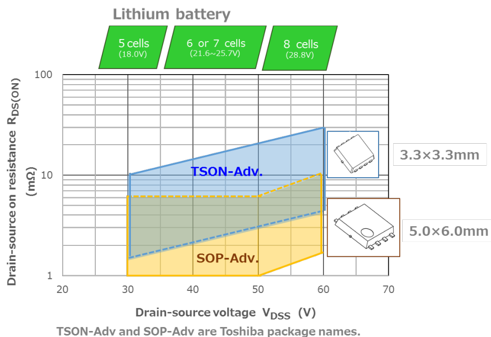
Figure 2.21 V_{DS} and R_{DS(on)} ranges and packages of recommended power MOSFETs according to the battery voltage
