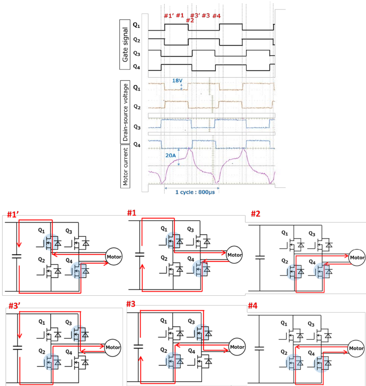
(b) Basic circuit operations and waveforms at a high suction level
