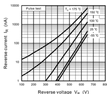
Figure 2.2 Example of I_R - V_R curve
