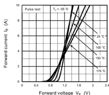
Figure 2.1 Example of SiC SBD I_F - V_F curve
