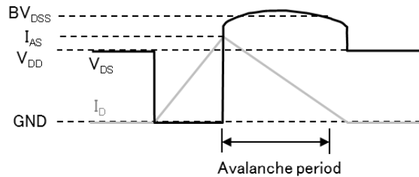
Figure 2.2 Avalanche waveform
