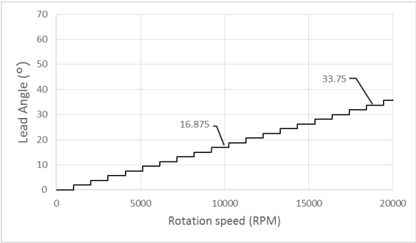
Figure 11.4 Example of the setting of lead angle LTABLE = 14 (1b01110)
