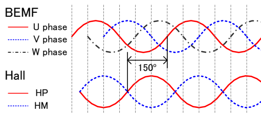
Figure 11.11 The waveform of Hall signal and induced voltage in CW
