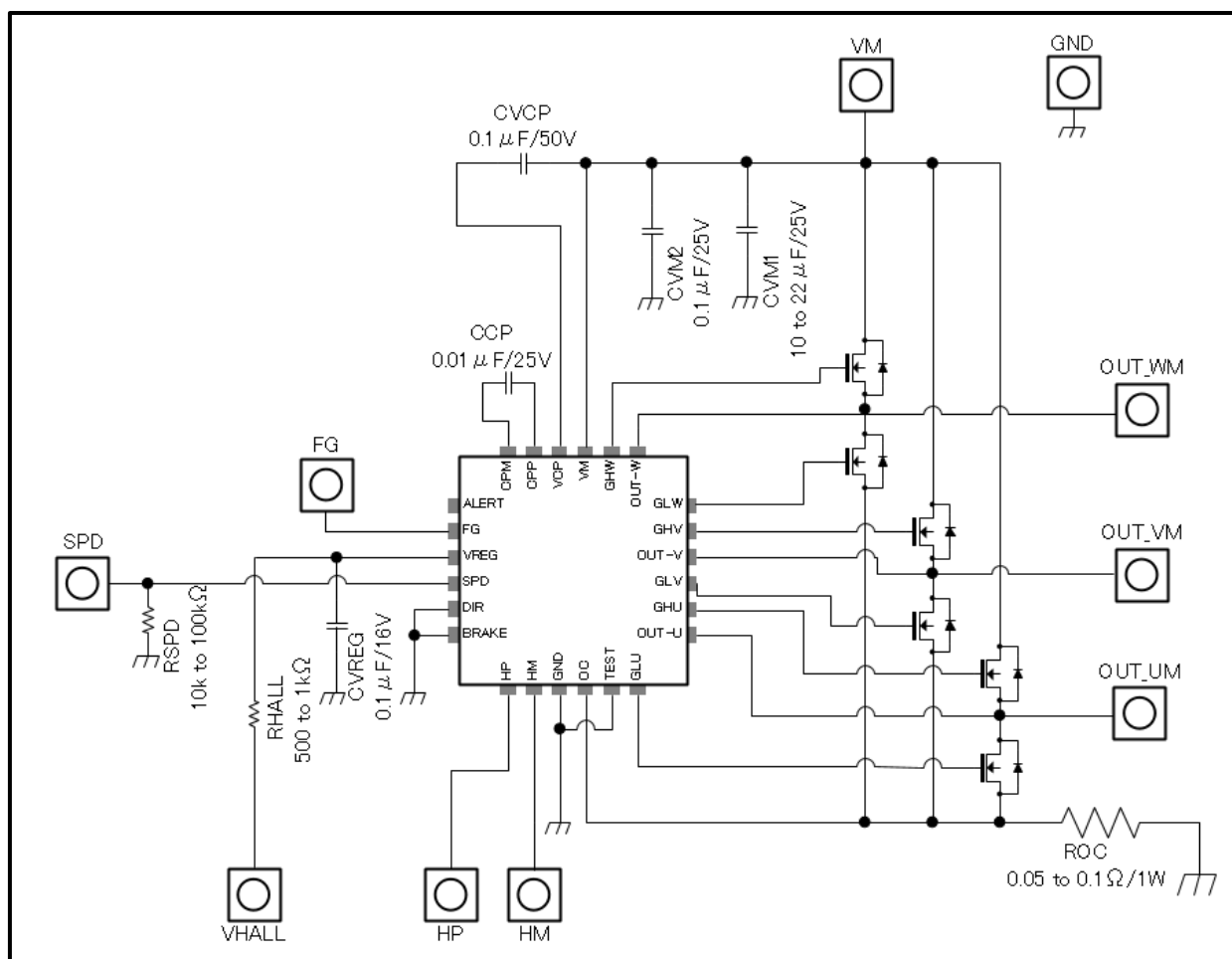
Figure 12.1 Reference circuit
