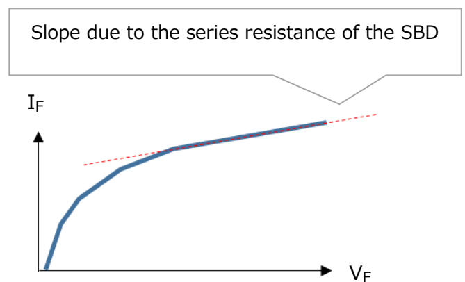
Figure 2-6 I_F - V_F curve of a conventional SBD
