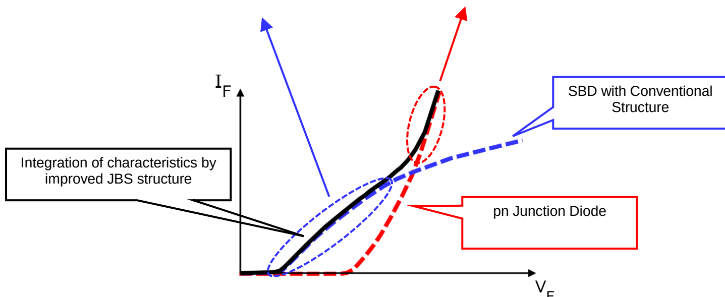
Figure 2-9 I_F - V_F curve
