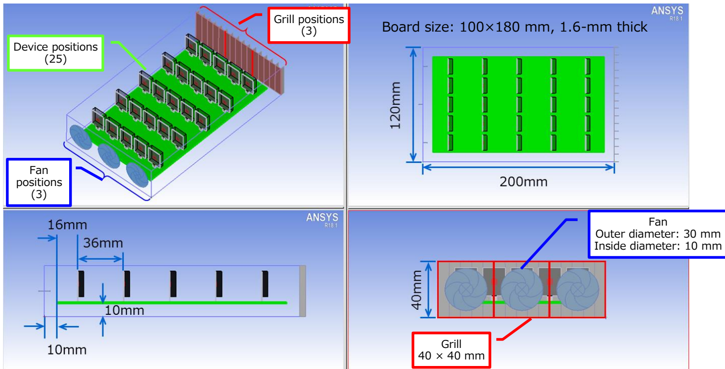
Figure 1 Simulation model 1
