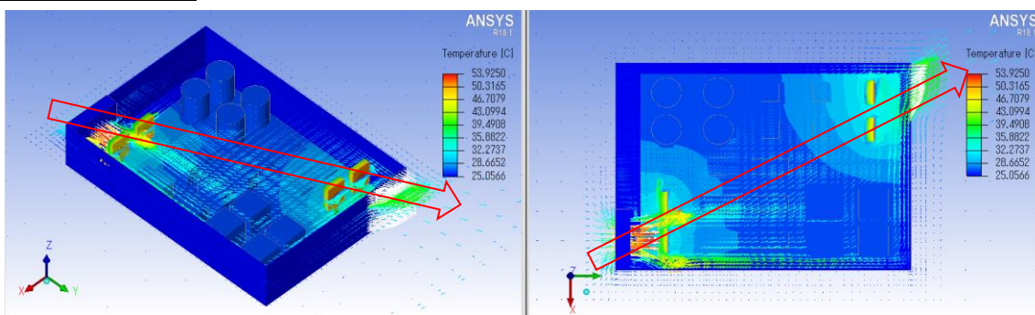
Figure 10 Temperature and air velocity distributions across Model 2 with a blower fan A
