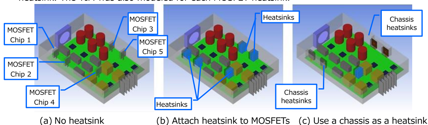
Figure 29 Simulation models:
