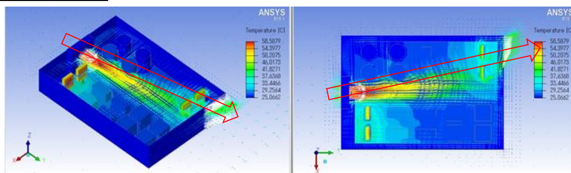
Figure 11 Temperature and air velocity distributions across Model 2 with a blower fan B
