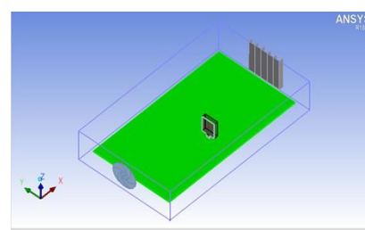
Model with Fan B, Grill B, and MOSFET C2
