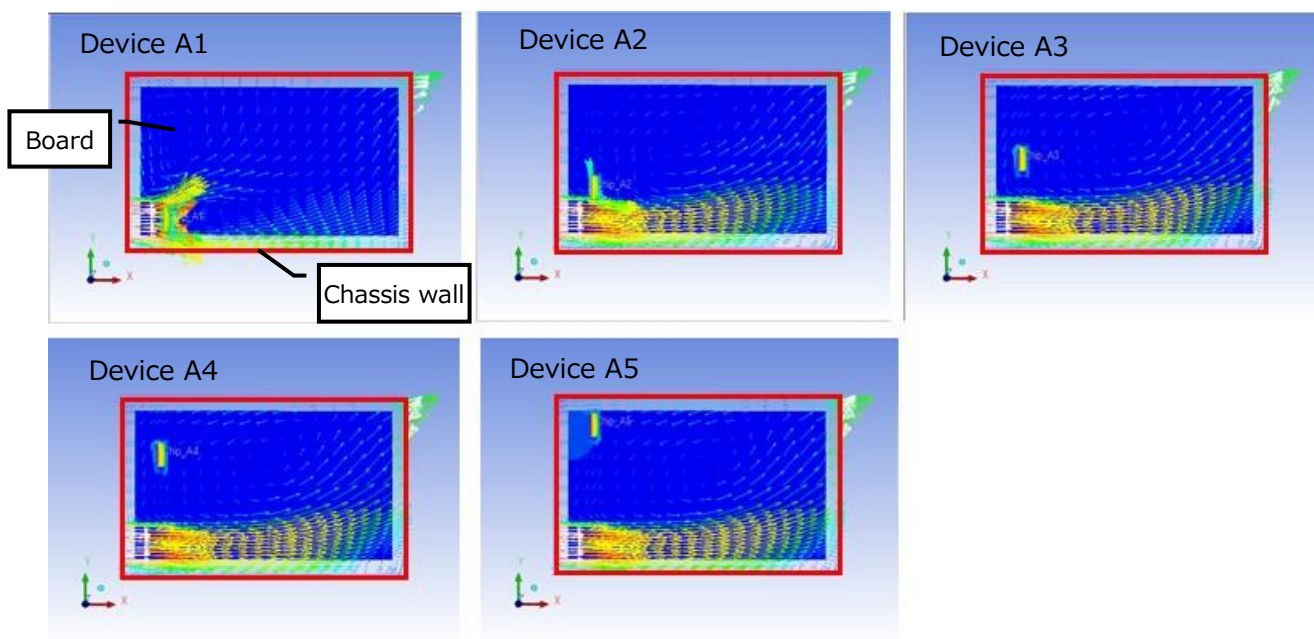
Figure 6 Airflow from Fan A to Grill C (Only the vector direction is shown for the outside of the chassis.)
