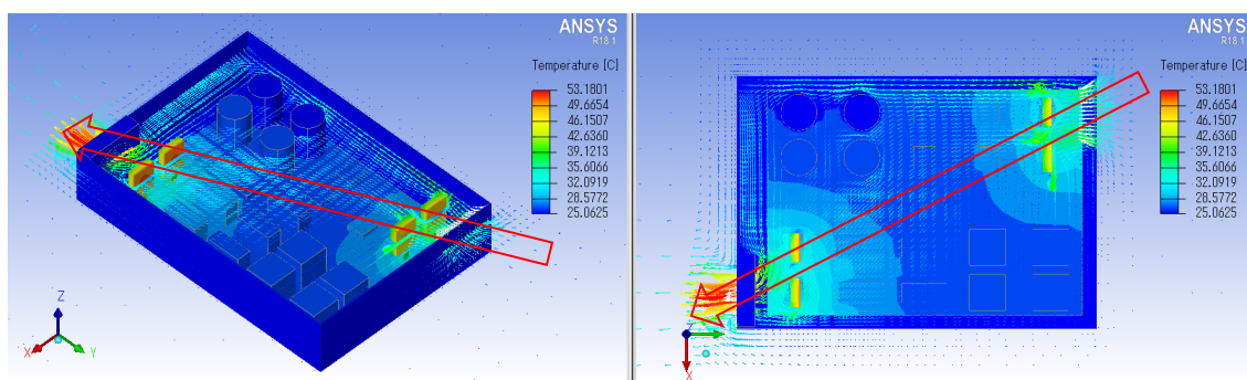
Figure 13 Temperature and air velocity distributions across Model 2 with a suction fan A
