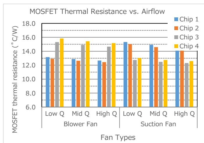
Figure 25 Comparison of the effects of fan performance on the MOSFET thermal resistance
