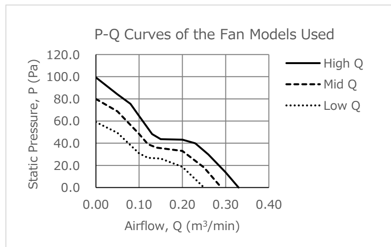
Figure 23 P-Q curves of the fan model
