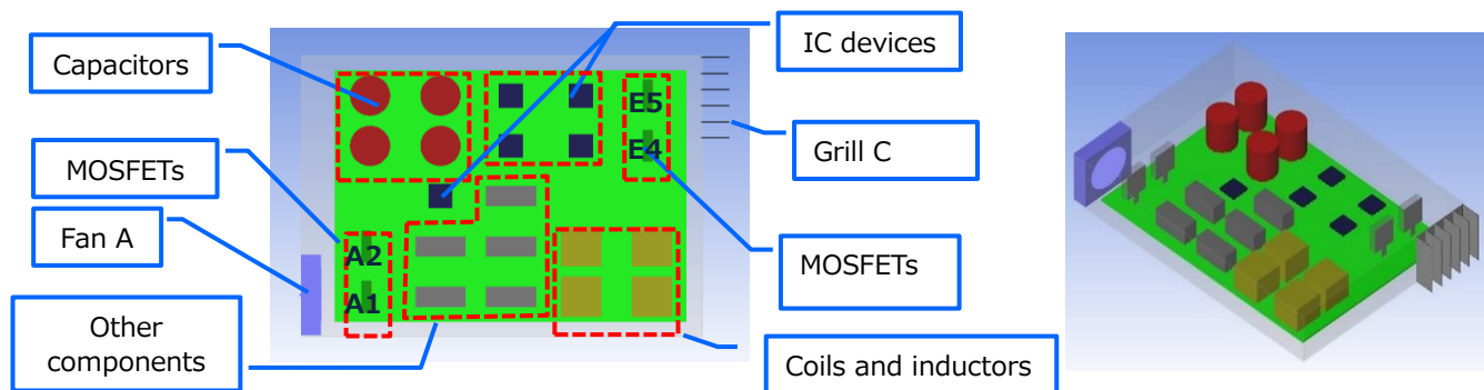
Figure 9 Component placement
