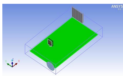
Model with Fan A, Grill C, and MOSFET B4
