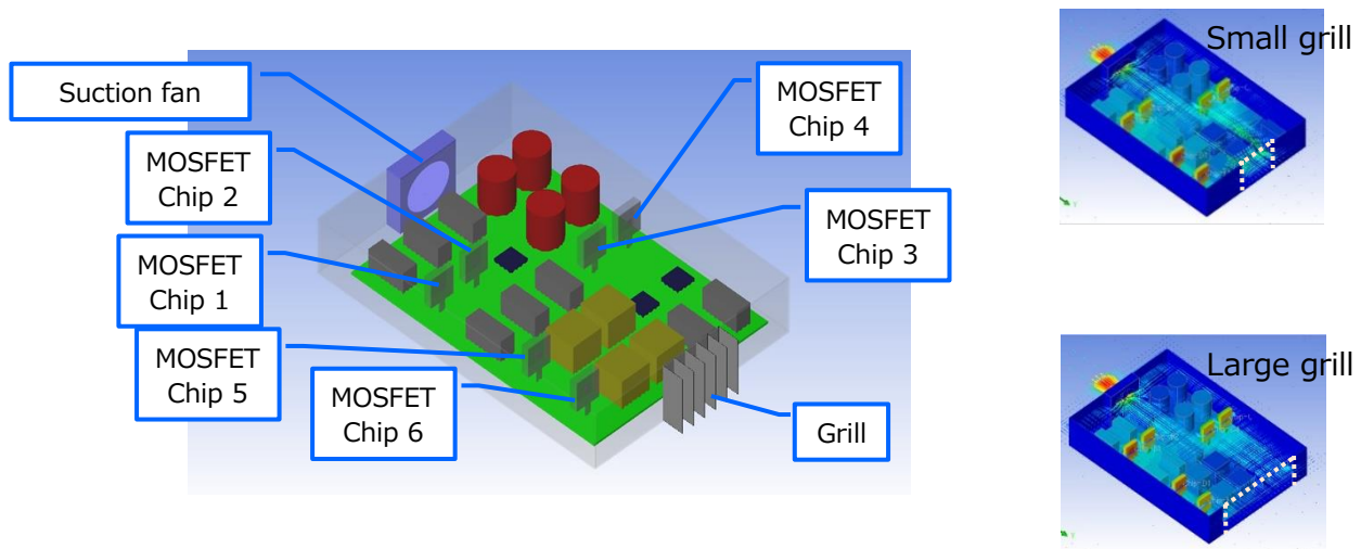
Figure 16 Model for the evaluation of the grill size
