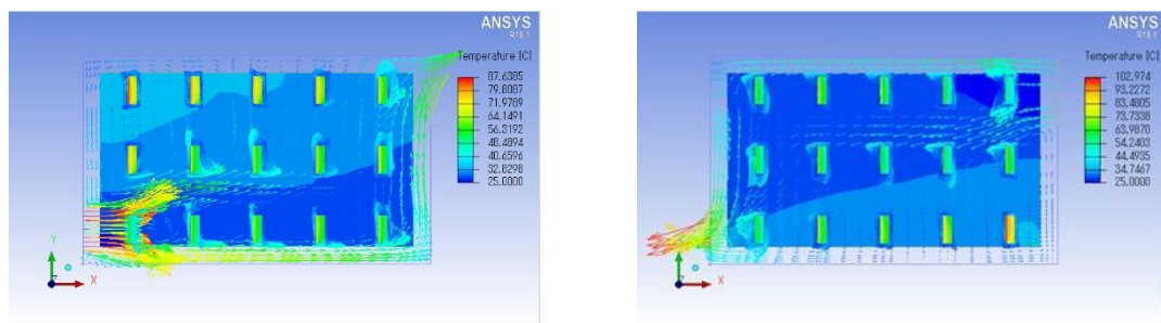
Figure 8 Thermal resistances of widely spaced MOSFETs: Blower fan (left), suction fan (right)
