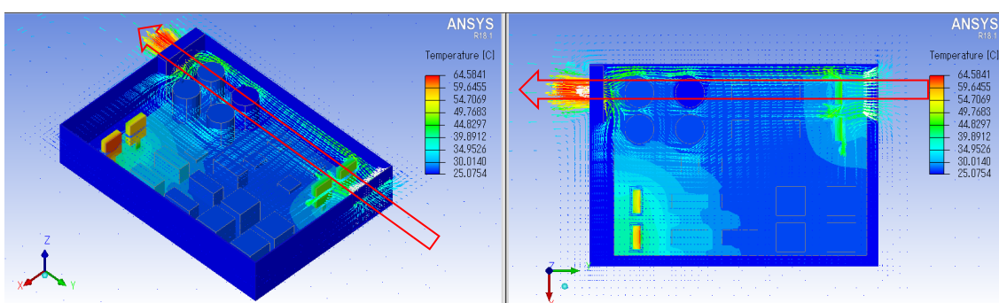
Figure 15 Temperature and air velocity distributions across Model 2 with a suction fan C
