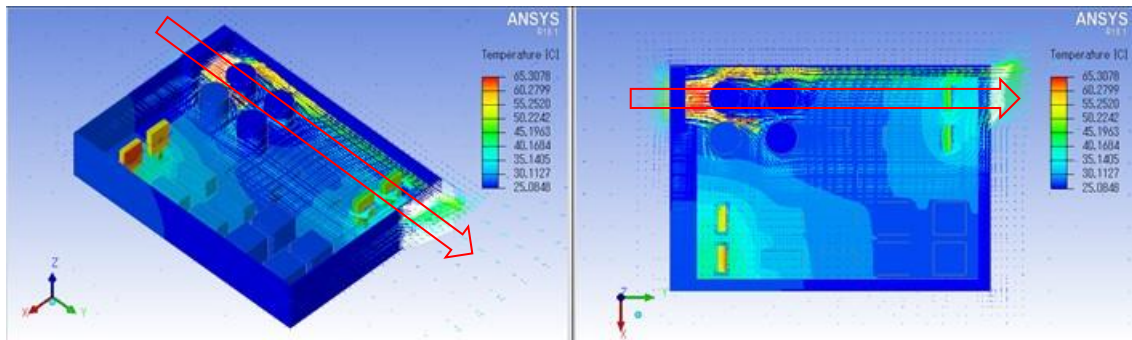
Figure 12 Temperature and air velocity distributions across Model 2 with a blower fan C
