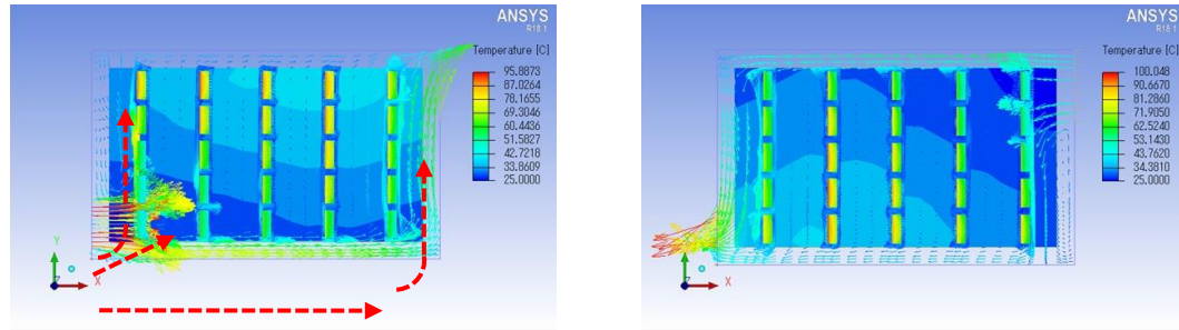
Figure 7 Temperature and air velocity distributions in a model with 25 MOSFETs: Blower fan (left), suction fan (right)
