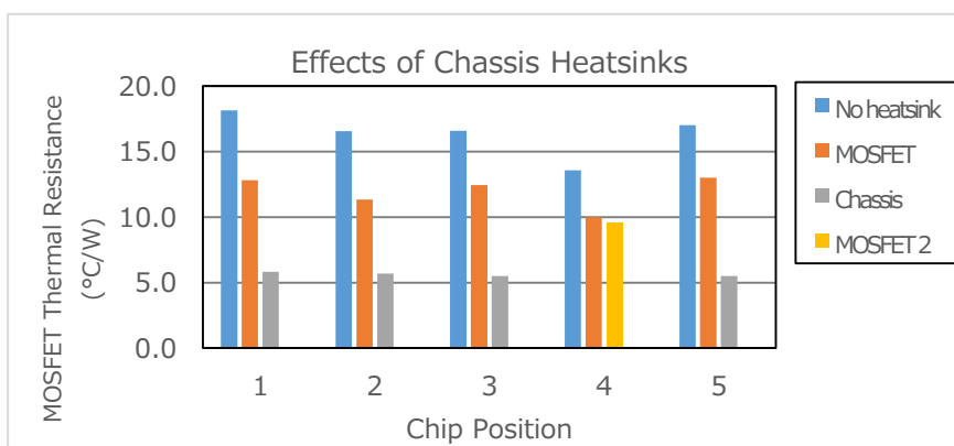
Figure 30 Effects of chassis heatsinks
