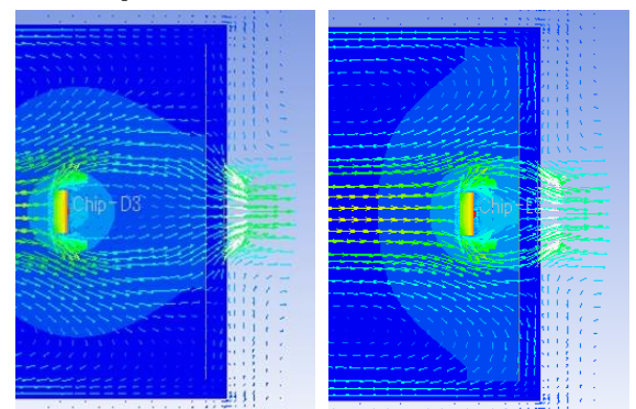
Figure 22 Airflow at the back of the MOSFET
