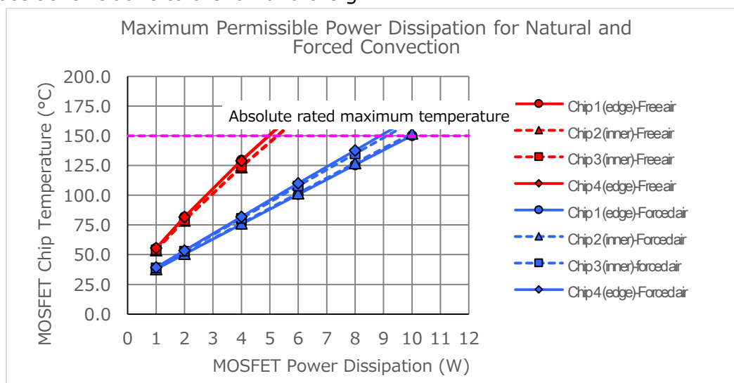
Figure 19 MOSFET chip temperatures in the case of natural and forced convection
