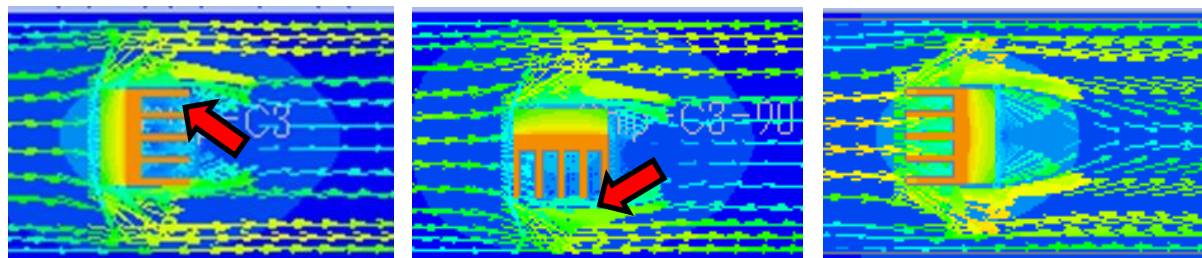
Figure 28 Air velocity distribution around the heatsink
