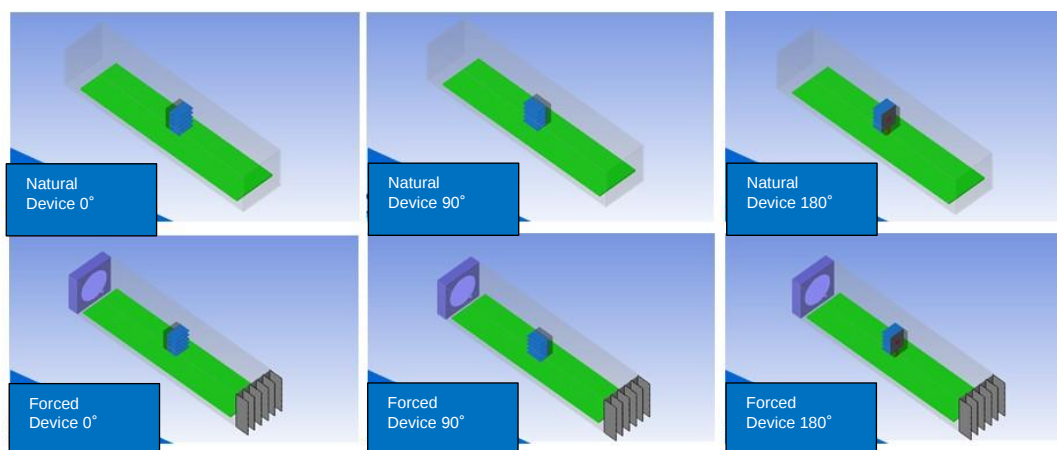
Figure 27 Simulation models used to evaluate the effects of heatsink orientations
