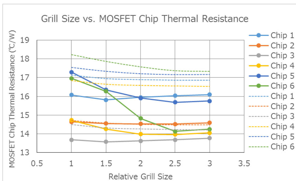
Figure 17 MOSFET thermal resistance vs. grill size
