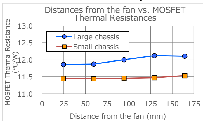
Figure 21 MOSFET thermal resistances vs. fan-to-MOSFET distances
