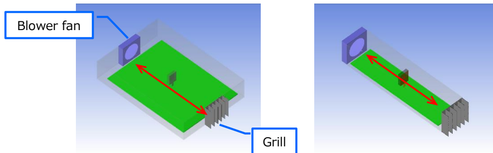
Figure 20 Simulation models used to evaluate the effects of the fan-to-MOSFET distances (with fixed fan and grill sizes)
