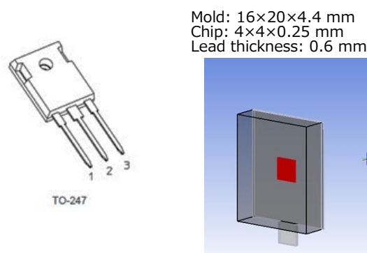
Figure 4 MOSFET shape (left) and simplified model (right)
