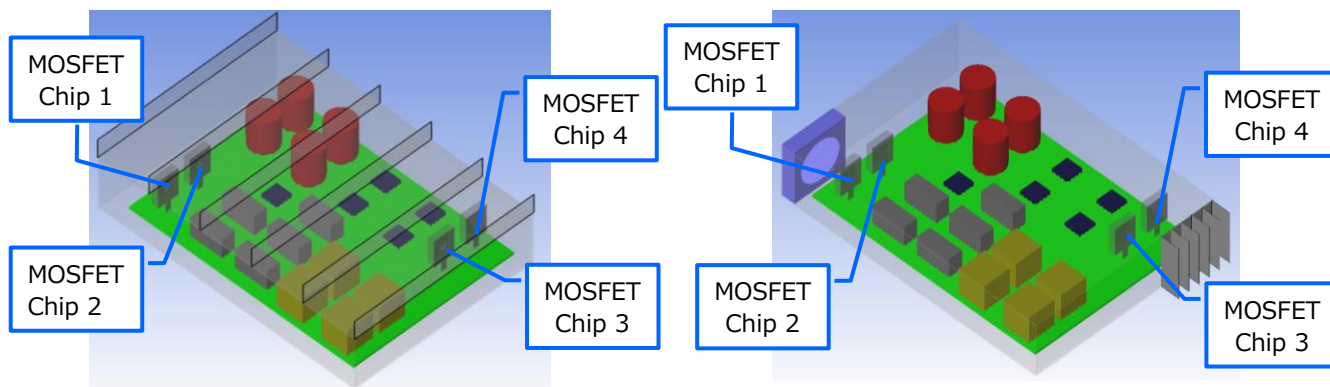
Figure 18 Natural-convection model (left) and forced-convection model (right)
