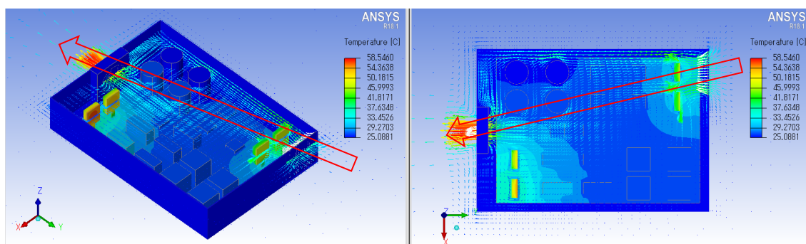
Figure 14 Temperature and air velocity distributions across Model 2 with a suction fan B
