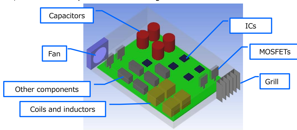
Figure 3 Simulation model 2 (example)
