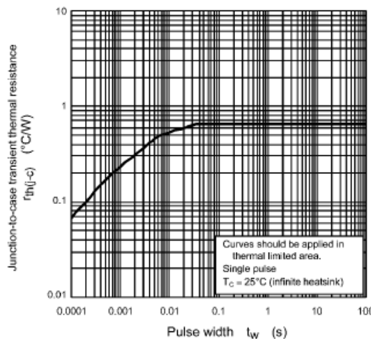
Figure 3.1 Transient thermal impedance curve
