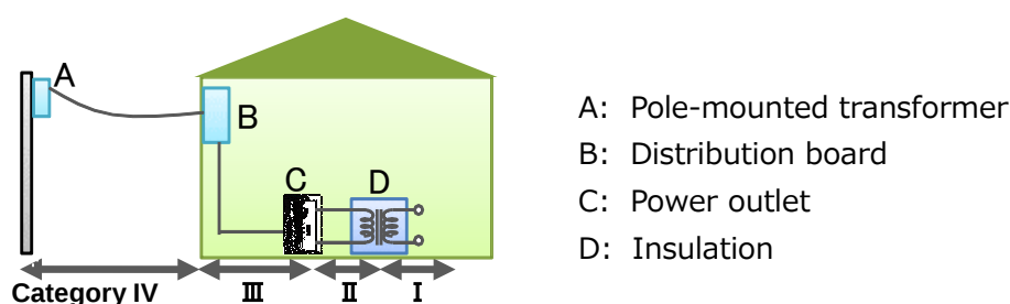
Figure 4.1 Overvoltage categories
