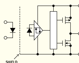
Active-Low IPM
