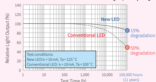
Estimated LED Aging Degradation ( \bar{X}-3\sigma )
