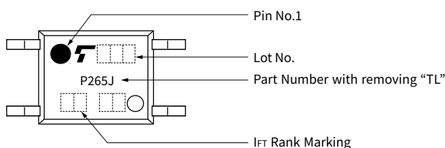
TLP265J (4 pin SO6 Package)
