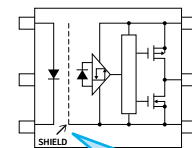
Electrostatic shielding for the photosensor chip provides a CMTI of 10 kV/ \mu s or higher.
