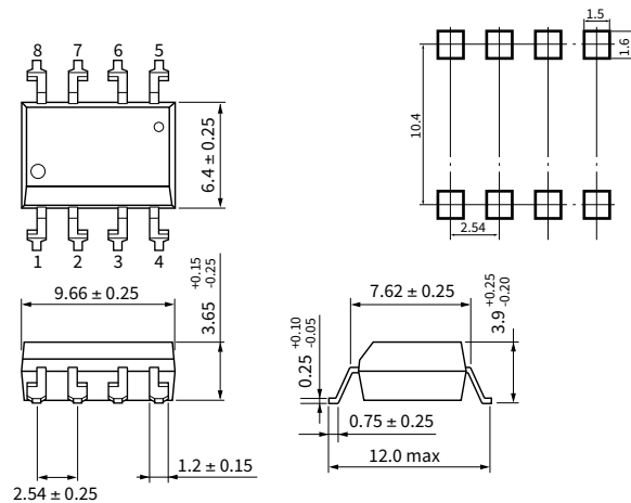
DIP8 (LF4)
