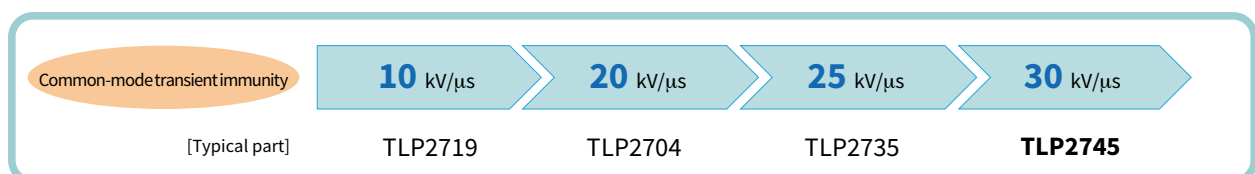
Electrostatic shielding for the photosensor chip provides a CMTI of 10 kV/ \mu s or higher.
