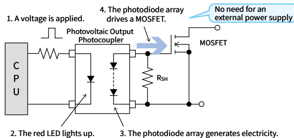
Example of a Circuit Composed of a Photovoltaic Output Photocoupler and a MOSFET
