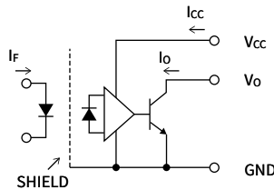
Open-Collector Output
