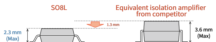
Comparison of the Package Height
