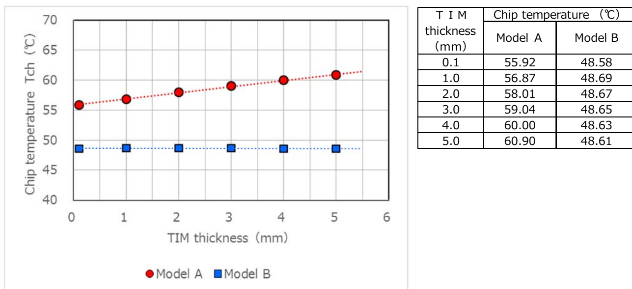
Figure 16 - TIM Simulation
