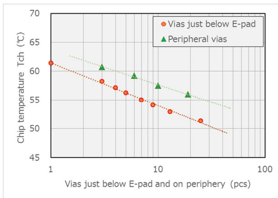
Figure 9 - Vias Just Below E-pad vs. Peripheral Vias
