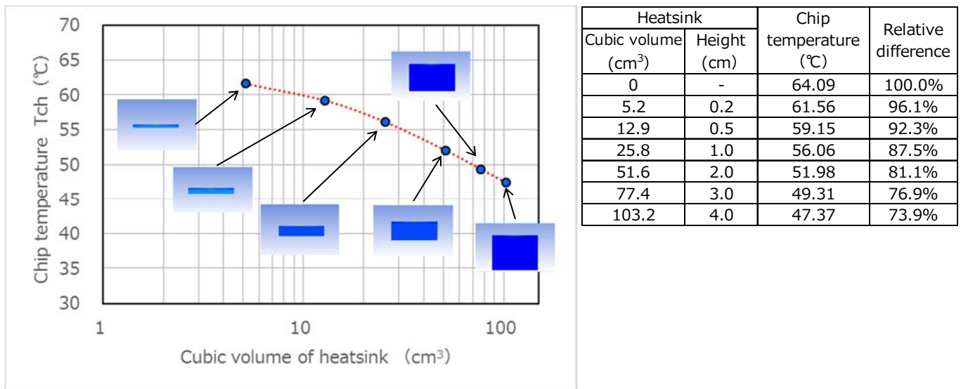
Figure 10 - Cubic Volume of Heatsink vs. Chip Temperature
