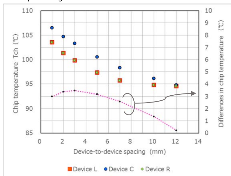
Figure 12 - Thermal Interference Simulation
