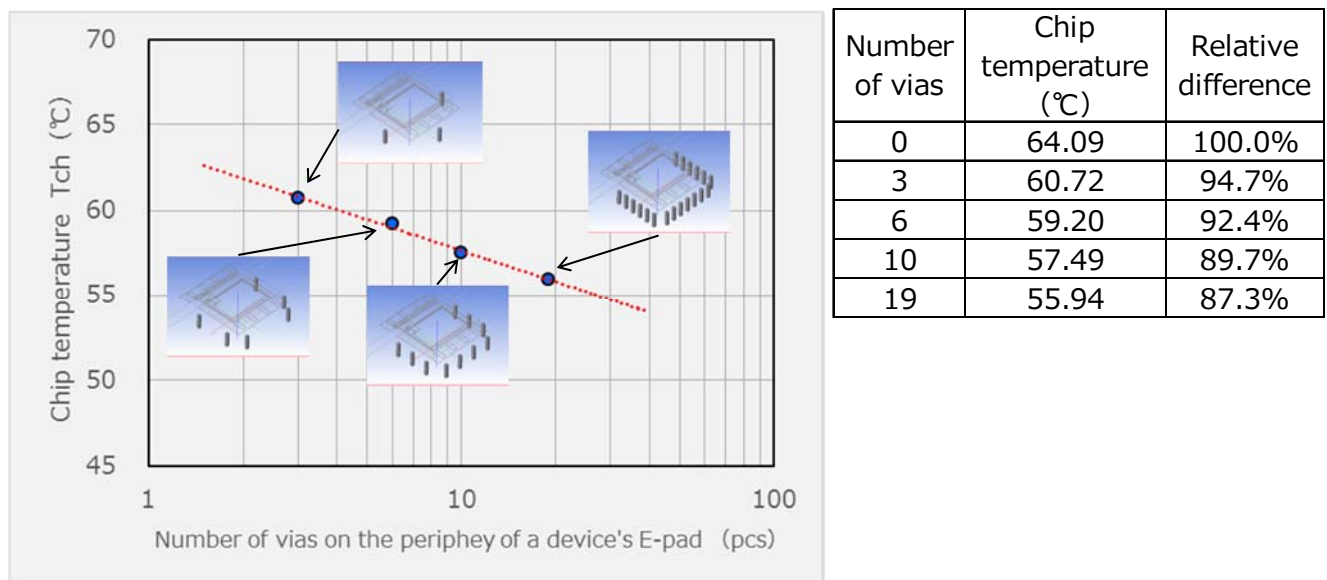
Figure 8 - Number of Vias on the Periphery of a Device's E-pad vs. Chip Temperature
