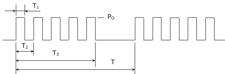
Figure 4.1 Intermittent, repetitive loss waveform
