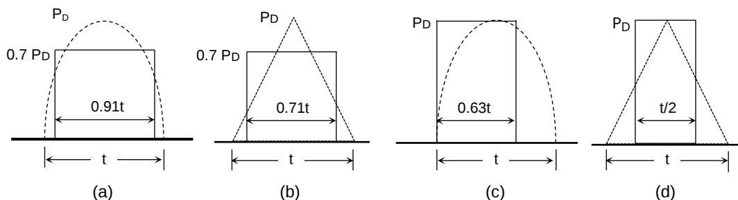
Figure 3.3 Waveform approximation
