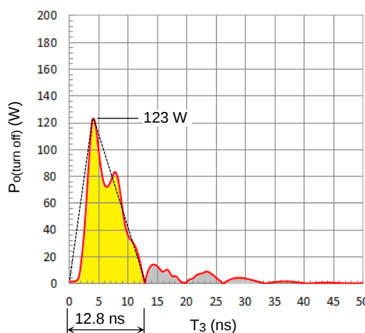
Figure 3.13 Turn-off loss waveform
