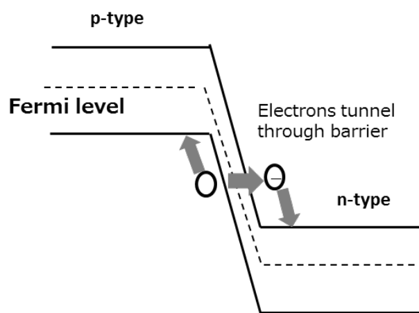
Figure 1.3 Zener breakdown
