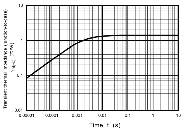
Fig. 9.5 r_{th(j-c)} - t (Guaranteed Maximum)
