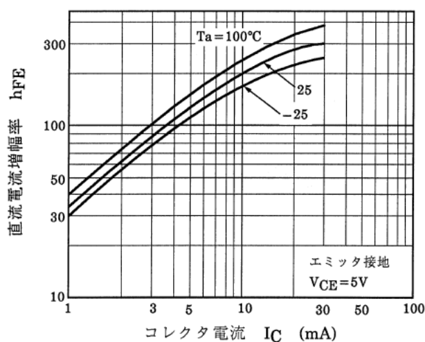
図 10.9 RN1909FE h_{FE}-I_C
