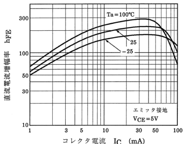
図 10.7 RN1907FE h_{FE}-I_C
