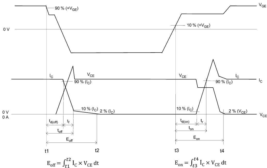
Fig. 6.2 Timing Chart
