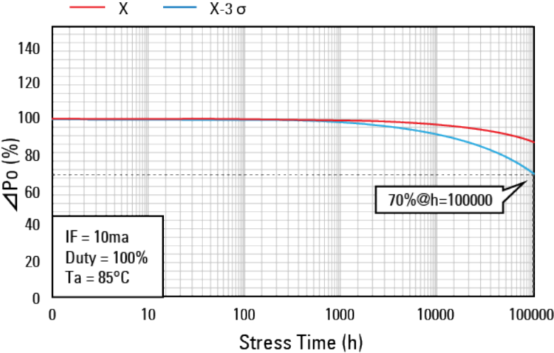
Fig. 1 GaAs LED projected light output degradation data
