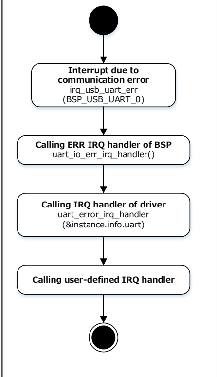
Interrupt calling flow chart
