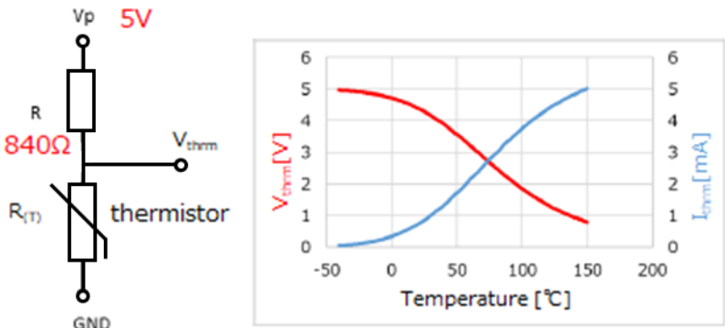
Fig. 9.3 An example of the circuit and output voltage and current for a thermistor
