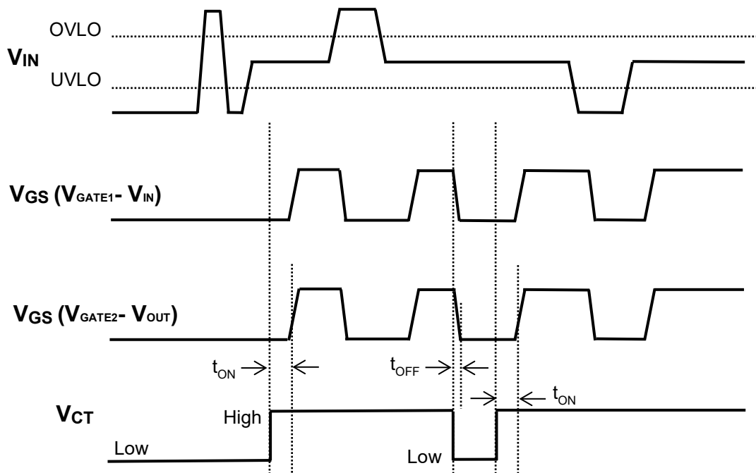
Fig.1 t_{ON} , t_{OFF}
