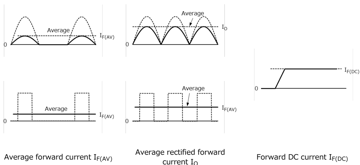
Figure 1.2 Definitions of steady-state current ratings
