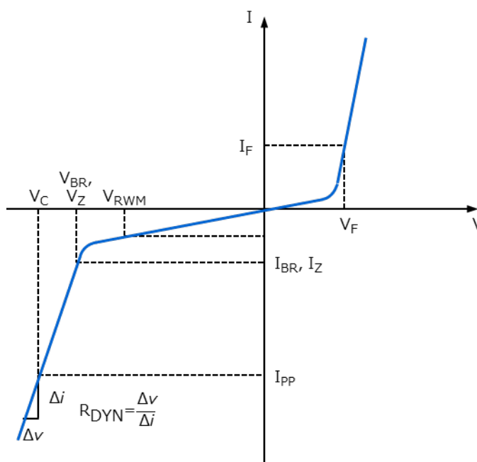
Figure 2-12 Definitions of electrical characteristics
