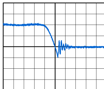
Figure 2.10 Example of an SBD recovery waveform Figure 2.11 Example of an HED recovery waveform
