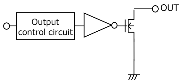
Fig.13 Open-drain with Inverted logic output circuit
