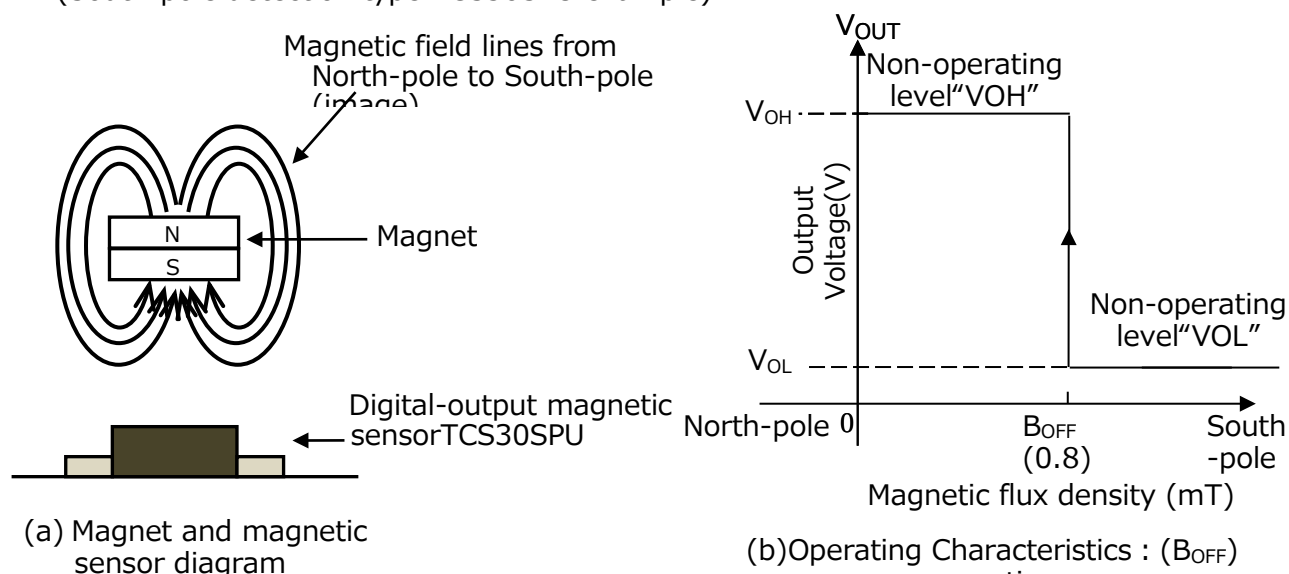
Fig.5 Operation characteristics as the magnet is brought away from the magnetic sensor. (South-pole detection type TCS30SPU example)
