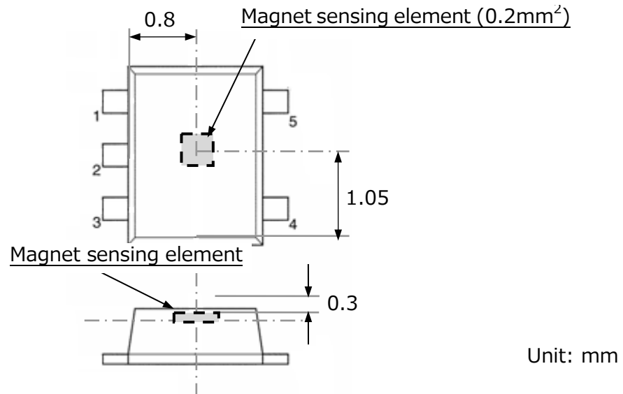
Fig.8 Magnet sensing element (South-pole detection type: TCS30SPU) : typical values
