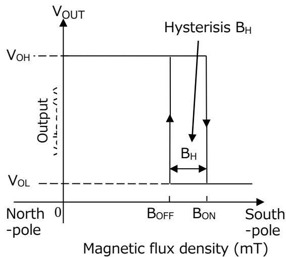
(b) Operating Characteristics
