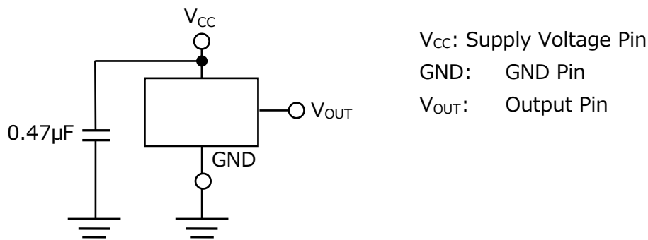
Fig.1 Basic operating circuit for Digital-output magnetic
