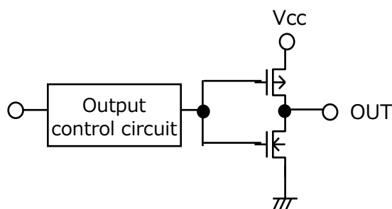
Fig.11 Push-pull output circuit
