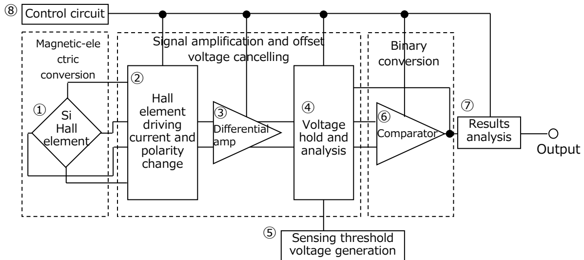
Fig.2 Digital-output magnetic sensor internal circuit block diagram
