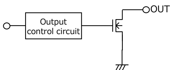
Fig.12 Open-drain output circuit
