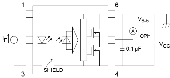
Fig. 13.1.1 I_{OPH} Test Circuit
