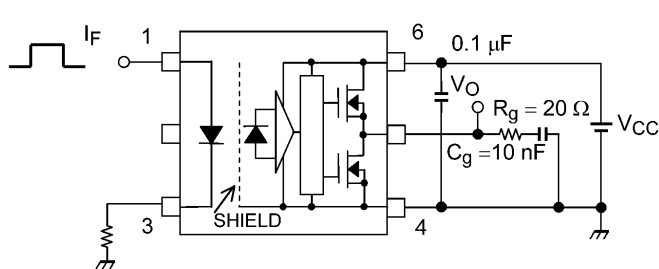
Fig. 13.1.7 Switching Time Test Circuit and Waveform
