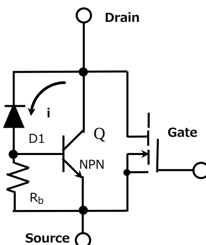
Figure 1.3 Equivalent Circuit Model for Avalanche Current
