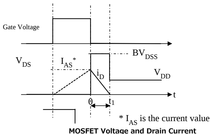
Figure 1.5 Waveforms During Avalanche Breakdown
