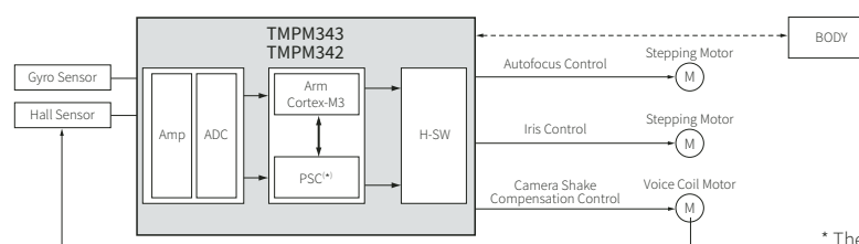
System Block Diagram (Camera Lens)
