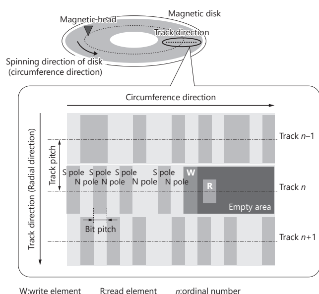
Figure 1. Outline of head and media of HDD
