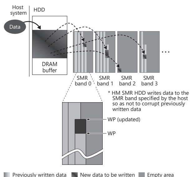
Figure 6. Data writing procedure in HM SMR HDD
