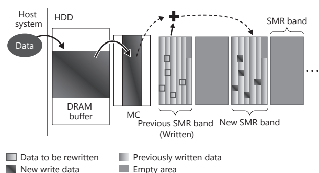
Figure 4. Data rewriting procedure in DM SMR HDD
