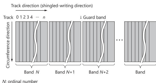
Figure 3. Configuration of shingled-written tracks and bands
