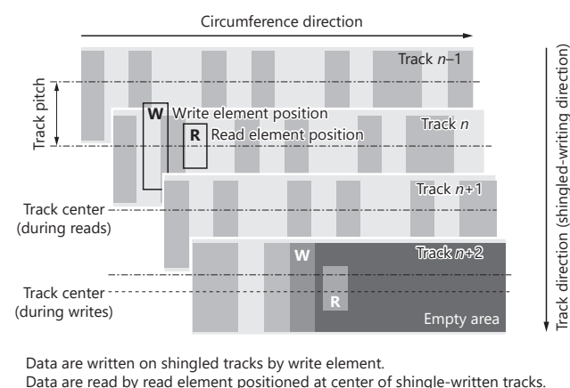
Figure 2. Schematic diagram of data tracks, write head, and read head of SMR HDD
