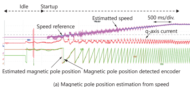
(a) Magnetic pole position estimation from speed
