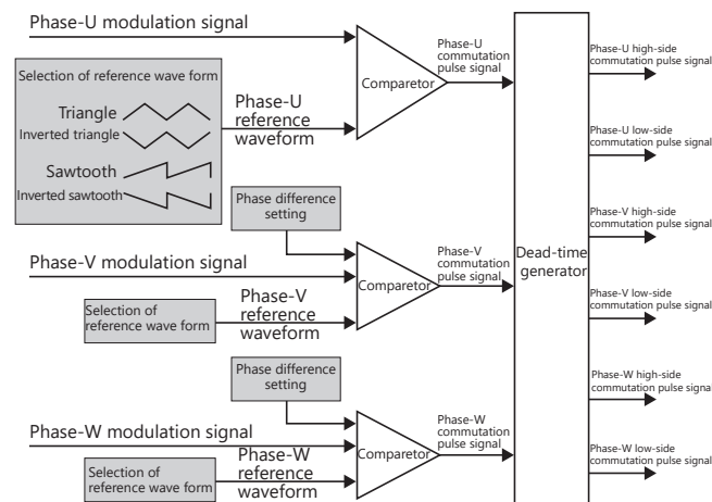
Figure 3. Pulse signal generation in A-PMD
