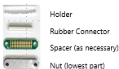
Fig.3 Connection Structure
