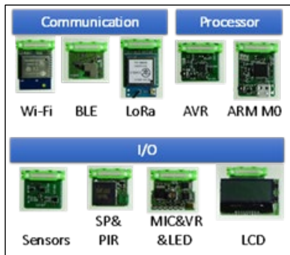
Fig. 2 Examples of leaf PCB
