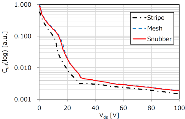
Fig.7 C_{gd} - V_{ds} curves of each structure at 100kHz.
