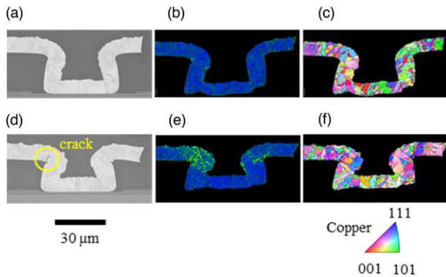
Fig. 14. (Color online) SEM image, orientation image (normal direction) and GROD maps of shallow via. (a)–(c) Initial, (d)–(f) after 1000 thermal cycles.
