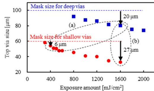
Fig. 7. (Color online) Relation between the exposure dose and via top diameter. (a) Multiple exposure process, (b) one-time process.
