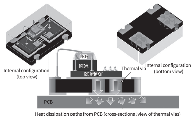
Figure 7. Structure and heat path of P-SON package
