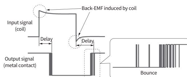
Figure 1. Switching waveform of mechanical relay
