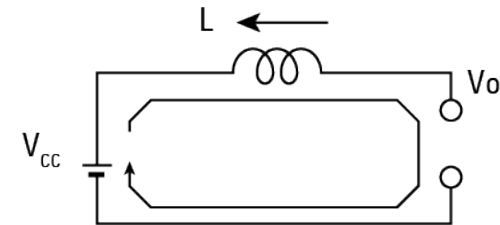
Reverse voltage: E = L \cdot (dI_L/dt)
