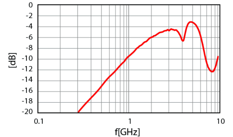
Insertion Loss: LED OFF
