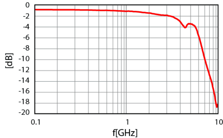
Insertion Loss: LED ON
